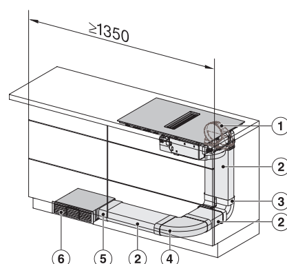
KMDA7272-1FL/FR, KMDA7473-1FL/FL MattFinish/ FR, KMDA7272FL/FR, KMDA7473FL/FR – Installation variant 2 Basis
