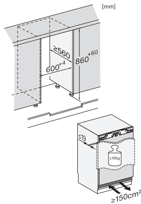
KU7135C, FNUS7140C, Built-under, niche dimensions
