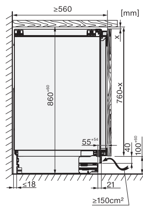
KU7135C, FNUS7140C, Built-under, side view
