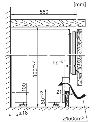
KU7135C, FNUS7140C, Built-under, side view
