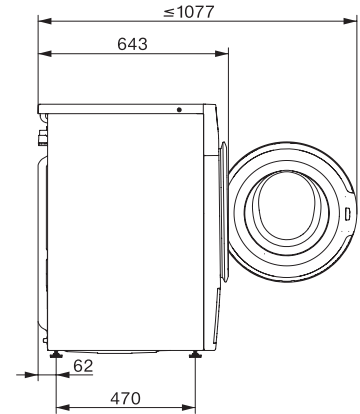
W1 drawing, fascia 5 degree, measures in mm
