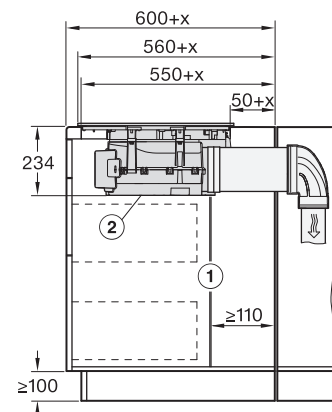
KMDA7676-1FL, KMDA7876-1FL – flush, drilling template, Installation depth 24,8 cm
