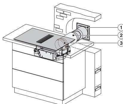
KMDA7676-1FL, KMDA7876-1FL – surface installation, 24,8 cm, drilling template
