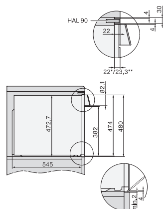
side view H7000 90 build-under, installation drawings
