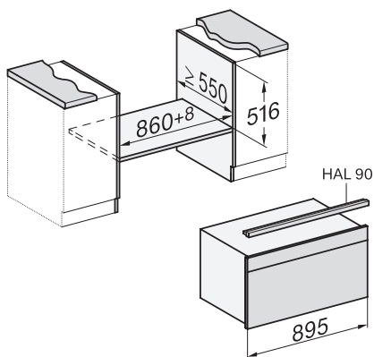
built-in H7000 90 build-under, installation drawing
